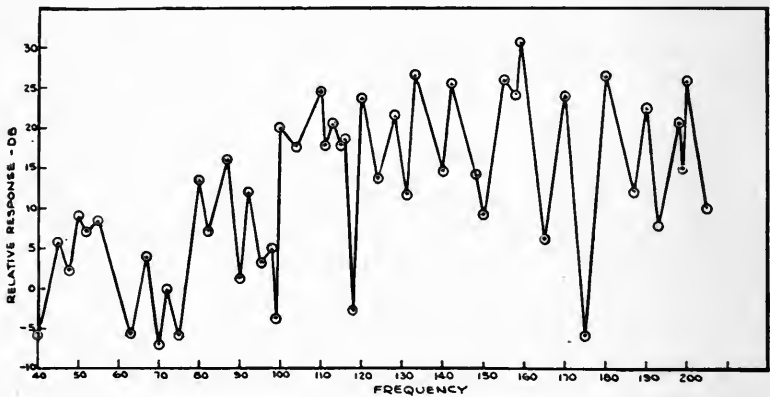
FIG. 1. Acoustical response measured in a small room, using sinusoidal signal.
